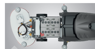
Interchangeable brush heads, so only one machine with different brush heads can be used instead of different machines
