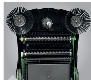
Fig. shows HKM 801 with tandem roller system
