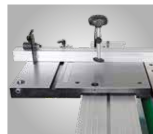
Sliding table with integrated scale. Mitre fence with one folding fence and one hold-down device.
